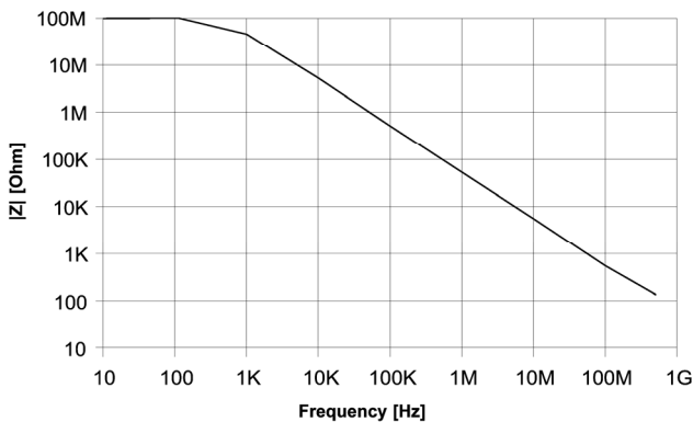
Typical Input Impedance PHV 4002-3
